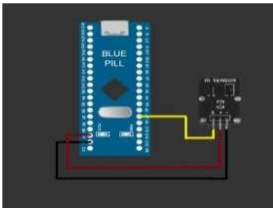
IR Sensor with STM32
